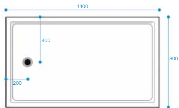
Tray not handed Reference Code: FALC1400x800
