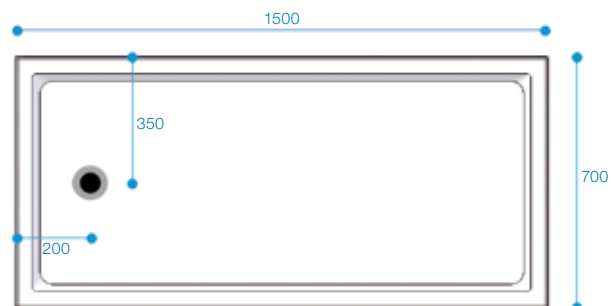
Tray not handed Reference Code: FALC1500x700
