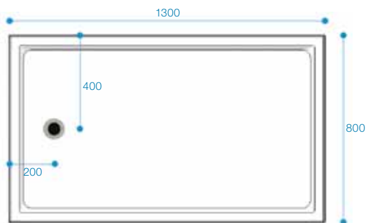
Tray not handed Reference Code: FALC1300x800
