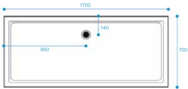
Tray not handed Reference Code: FALC1700x700
