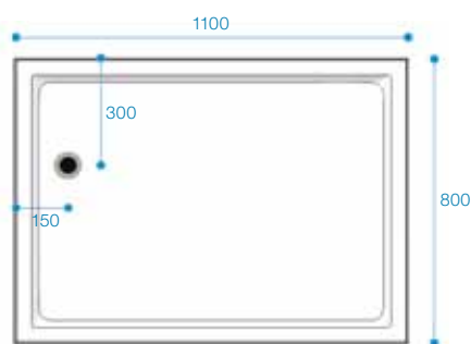
This tray has an offset waste position Tray not handed Reference Code: FALC1100x800
