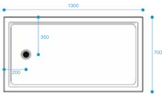
Tray not handed Reference Code: FALC1300x700
