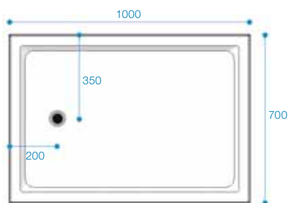
Tray not handed Reference Code: FALC1000x700
