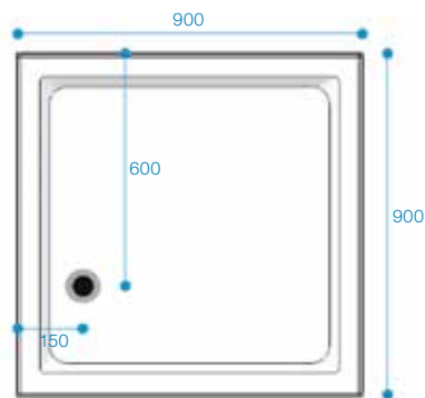
This tray has an offset waste position Tray not handed Reference Code: FALC900x900
