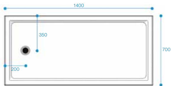
Tray not handed Reference Code: FALC1400x700
