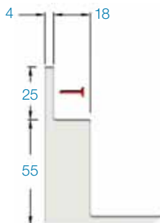
Tiling lip cross section
