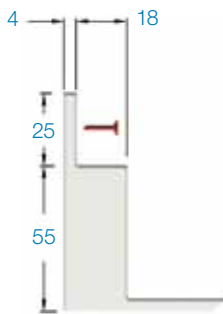
Tiling lip cross section
