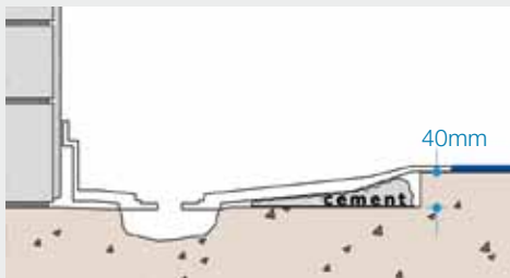
Void under the tray filled with a weak sand and cement mix
