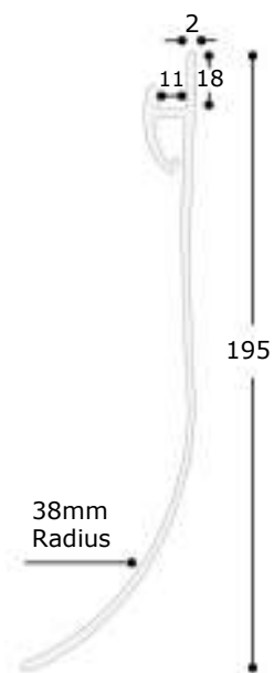
Coving creates a void, which can also be used for concealing plumbing
