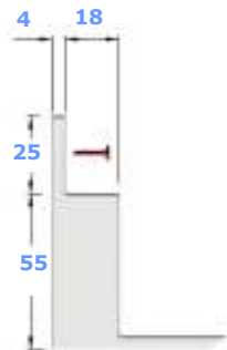
Tiling lip cross section
