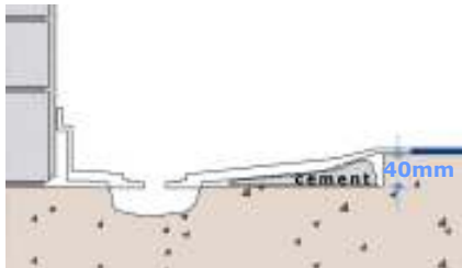
Void under the tray filled with a weak sand and cement mix
