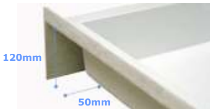
Void for concealed plumbing
