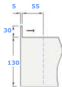
Tiling lip
