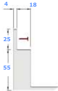
Tiling lip cross section
