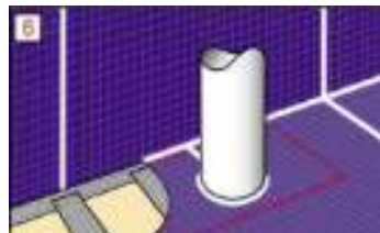
6 Tilesafe membrane is simple to detail around service entries and seal with either the supplied jointing compound or putty.
