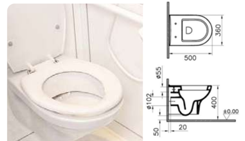
WC cubicles use a wall hung pan which allows cleaning underneath & around the WC.
