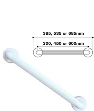
Straight fluted grab rails 300, 450 & 600mm
