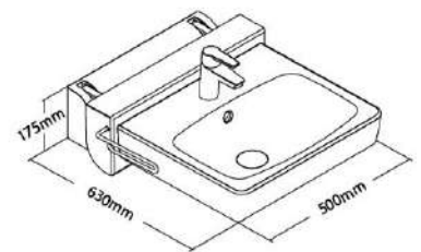
QuickWash placed in lower position
