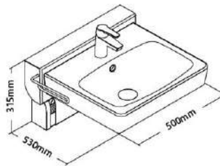
QuickWash placed in upper position
