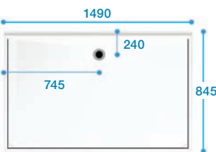
SIZE: 1490x845mm REF: SWIF1490 Not handed
