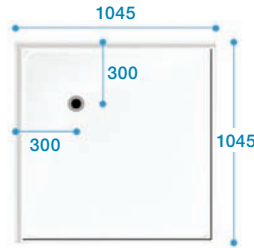
SIZE: 1045x1045mm REF: SWIF1045 Not handed
