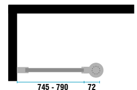
800mm shower screen with grab pole illustrated.
