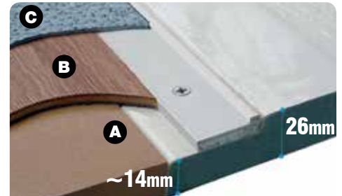
A - Floorboard or concrete flooring B - 1/4" plywood C - 2mm vinyl sheet flooring
